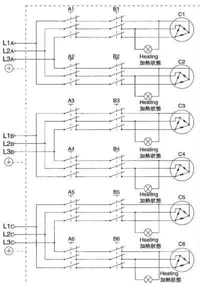
六組發熱芯 6 set Heating element 380V3~
